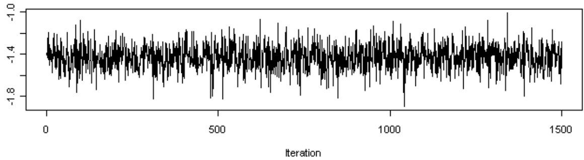
History of chain iterations for Beta3
