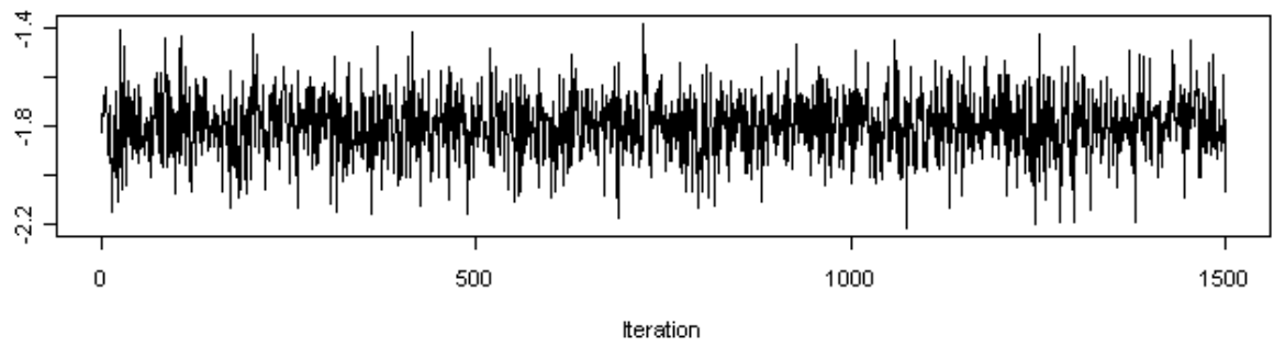
History of chain iterations for Beta2
