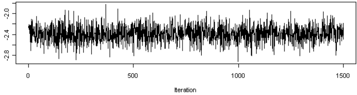
History of chain iterations for Beta1
